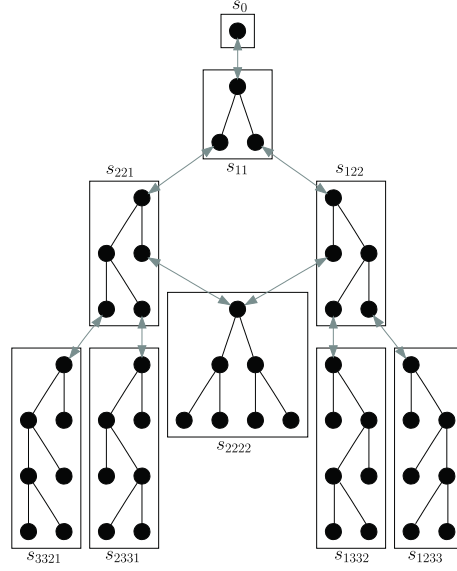
Fig. 2. Transition diagram over \mathbb{S}_{0,3} with split/reunion transitions from one RP state to another.
